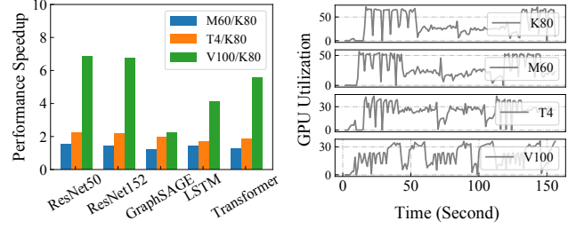
Figure 2: Training speedup of different jobs on different GPUs.
