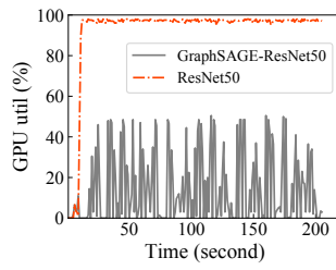
Figure 8: V100 GPU utilization with and without task switching.
