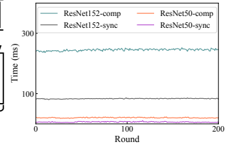
Figure 11: Training two popular models on 8 V100 GPUs.
