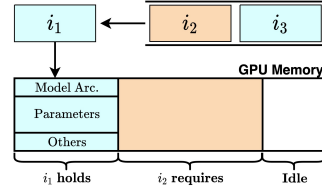
Figure 10: An example of speculative memory management.
